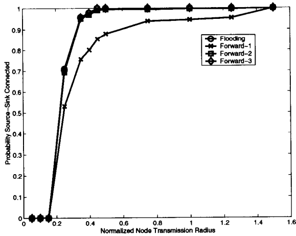
Fig. 4. Probability that a route exists with respect to Transmission Radius (5 % failure rate)
