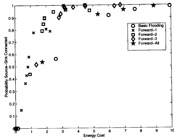
Fig. 7. Probability that a route exists with respect to normalized energy cost (20 % failure rate)
