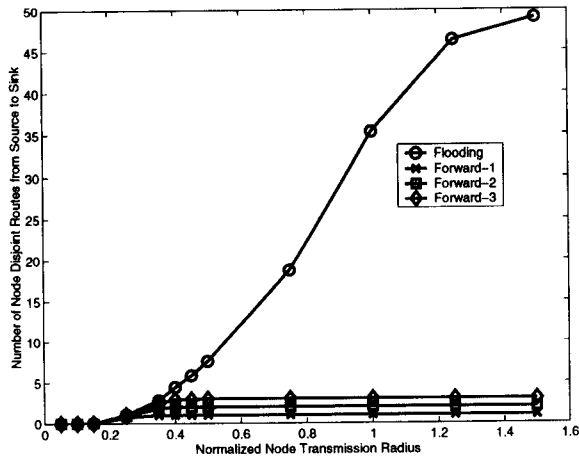
Fig. 2. Number of Node Disjoint Source Sink Routes with respect to the Transmission Radius
