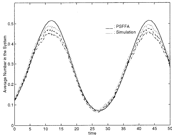
Figure 6: Comparison of the IPP/M/1 model with simulation for nonstationary traffic
