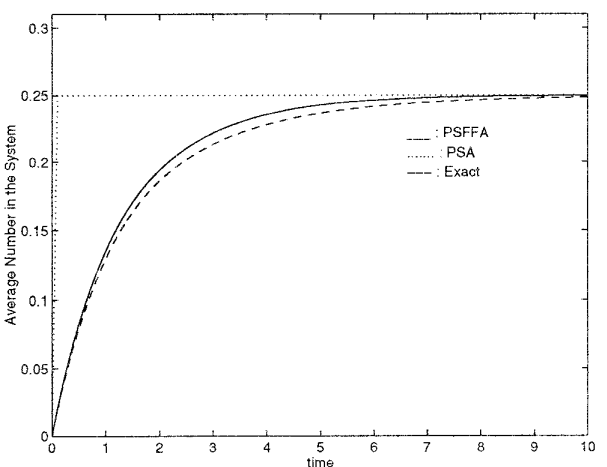
Figure 8: Comparison of the M/M/1/20 model transient behavior with exact solution
