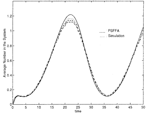
Figure 7: Comparison of the E_2/E_2/1 model with simulation for nonstationary traffic
