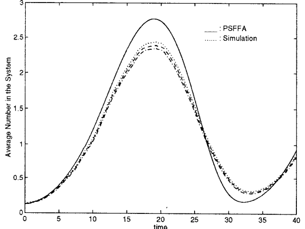
Figure 3: Comparison of the M/M/1 model with simulation for nonstationary traffic
