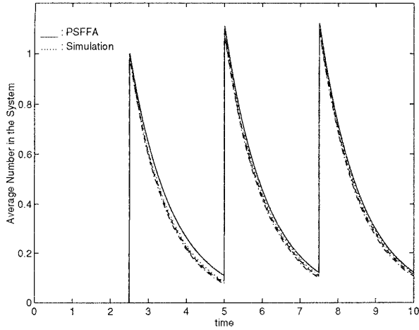
Figure 4: Comparison of the D/M/1 model with simulation for low load
