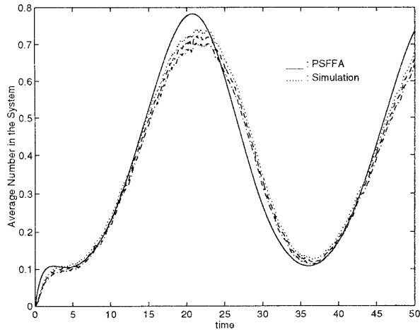
Figure 5: Comparison of the E_2/M/1 model with simulation for nonstationary traffic
