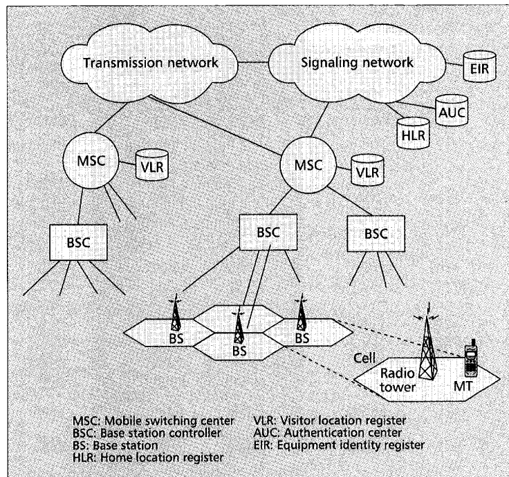
■ Figure 1. Wireless access network architecture.
