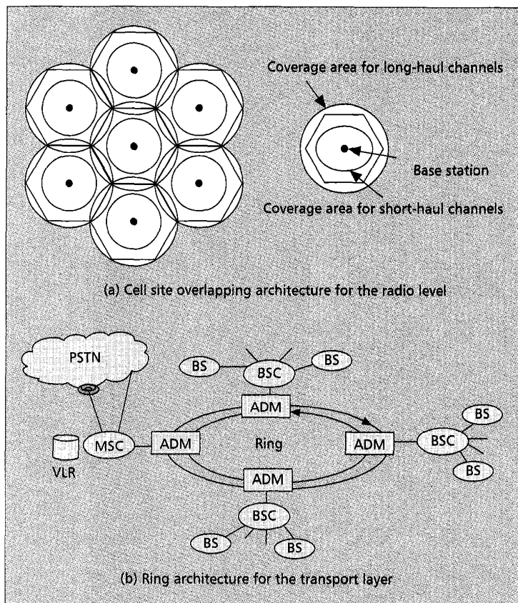
■ Figure 3. Survivability strategies for wireless access networks.
