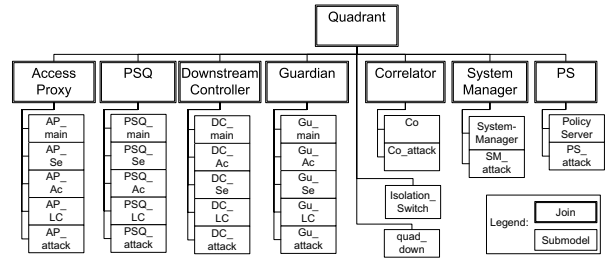
Figure 6. Quad Composed Model
