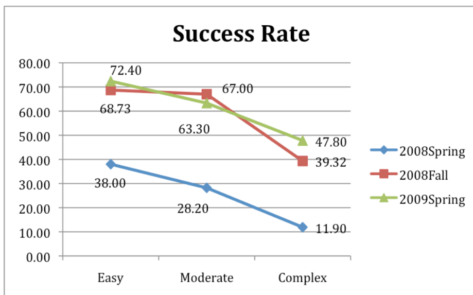
Fig 7. The Success Rate of two systems on different complexity levels; 2008Spring represents QuizJET; 2008Fall&2009Spring represent JavaGuide
