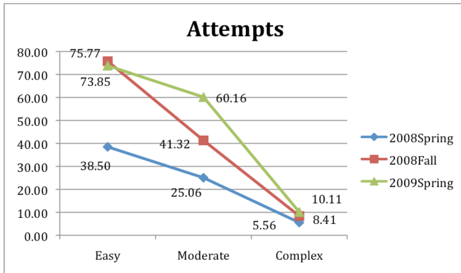
Fig 6. The total Attempts of two systems on different complexity levels; 2008Spring represents QuizJET; 2008Fall&2009Spring represent JavaGuide
