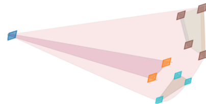
Figure 7. User-Defined Clusters
